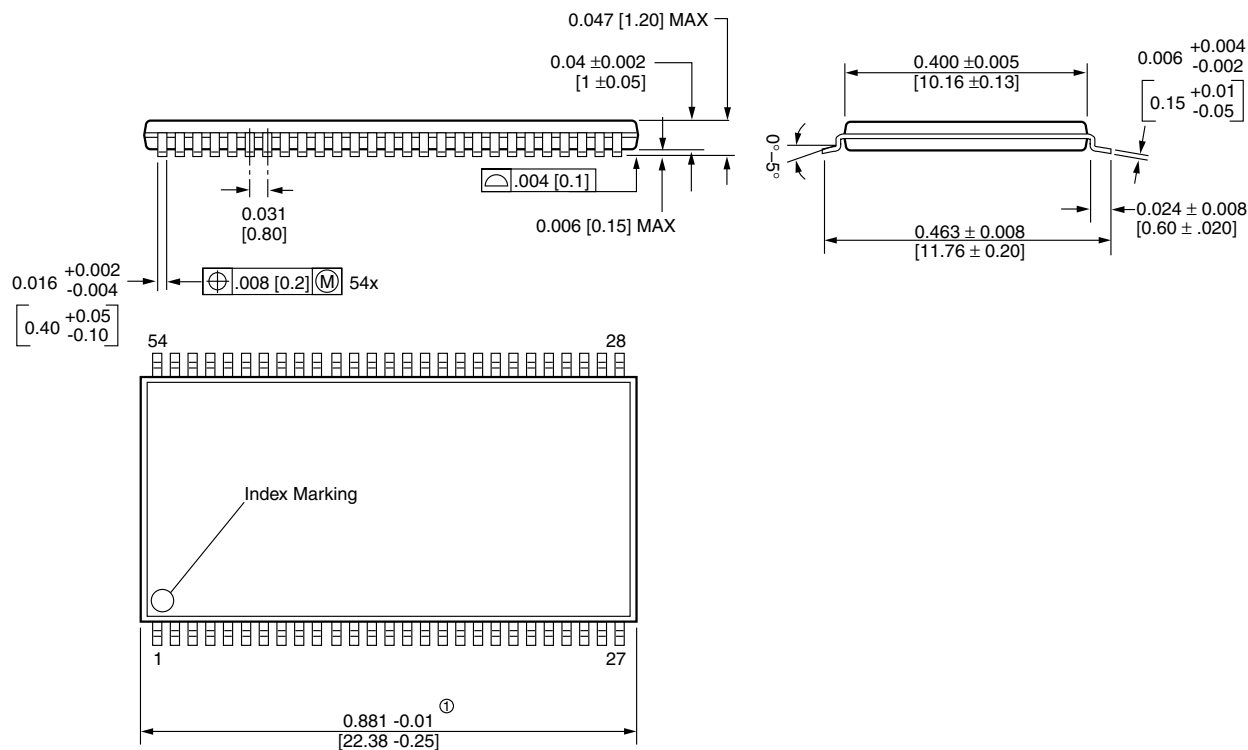
Package Diagram 54 PINS TSOP II
