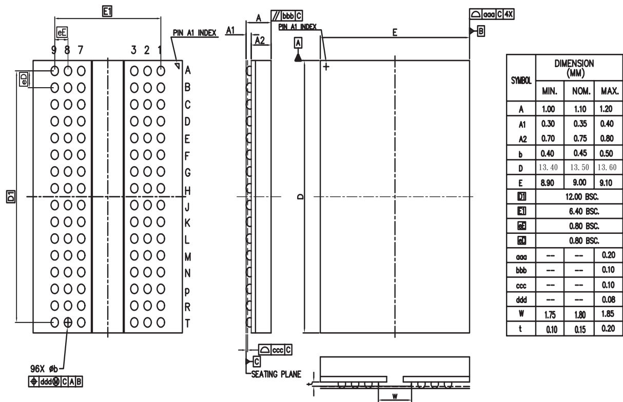
Package Diagram (x16)
